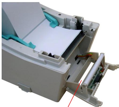
Backing paper opening
